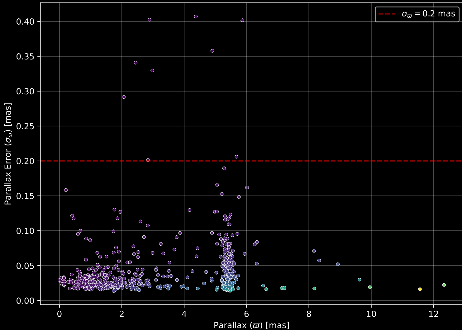
APOGEE DR17 Field: [NGC2632_btx] Parallax Quality (n= 548)
