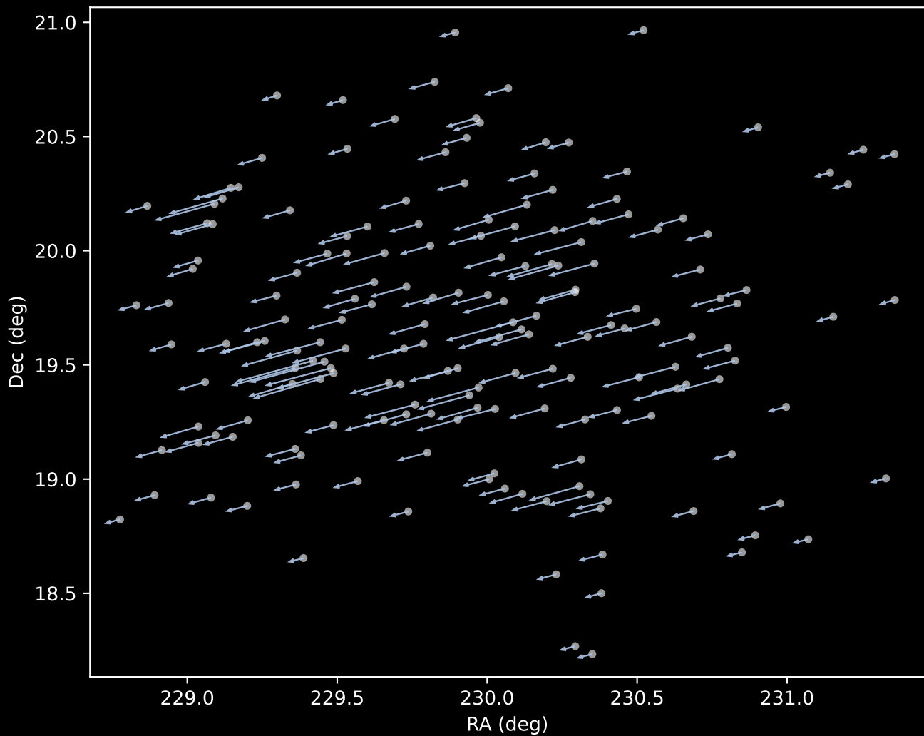
APOGEE DR17 Cluster 1 Proper Motion Vectors (n=178)
