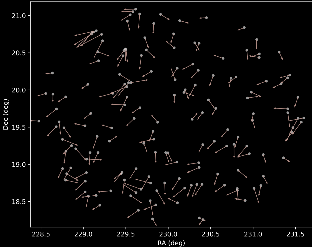
APOGEE DR17 Cluster 11 Proper Motion Vectors (n=162)
