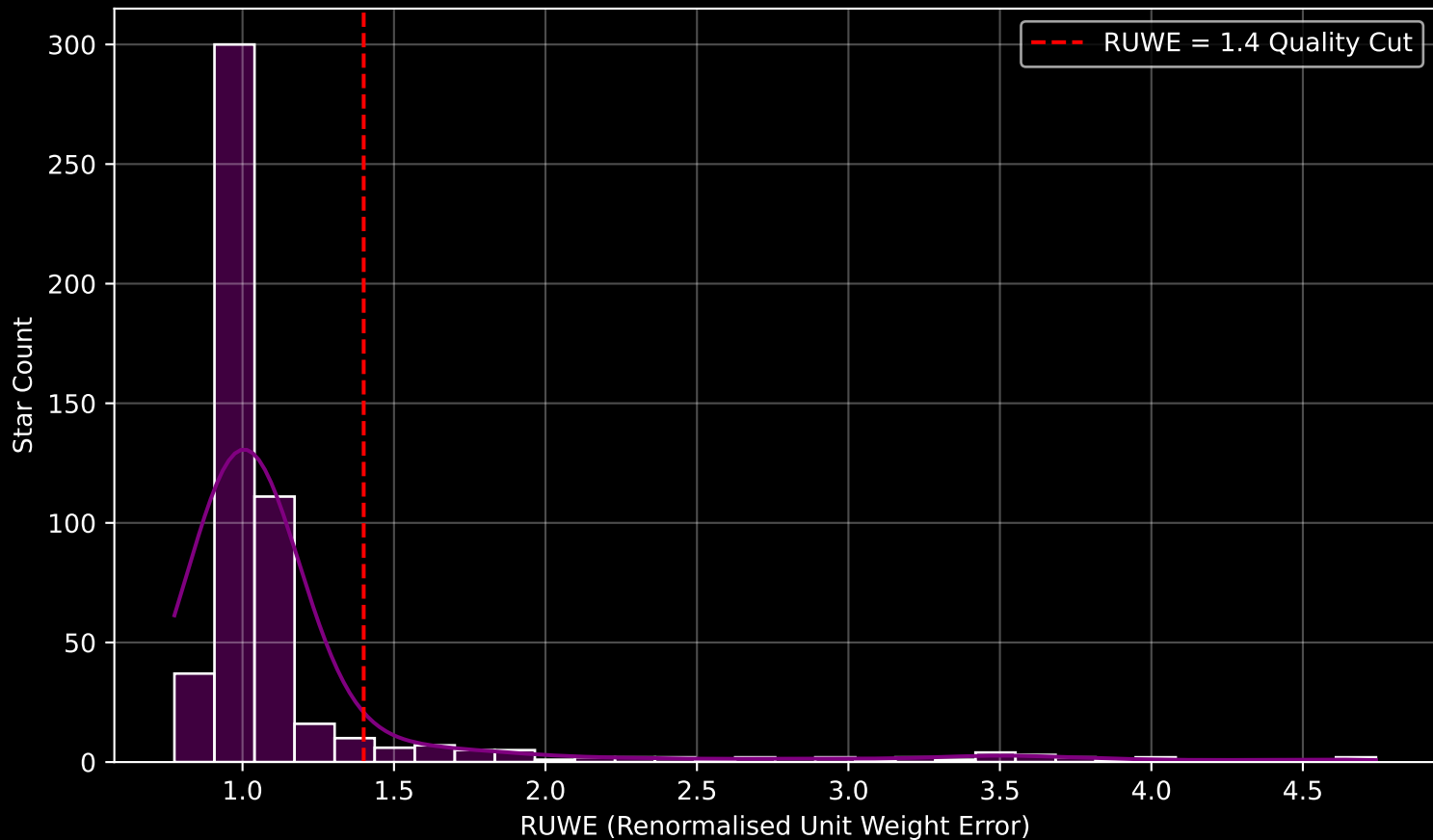
GAPOGEE DR17 Field [NGC2632_btx] RUWE Distribution (n= 530)
