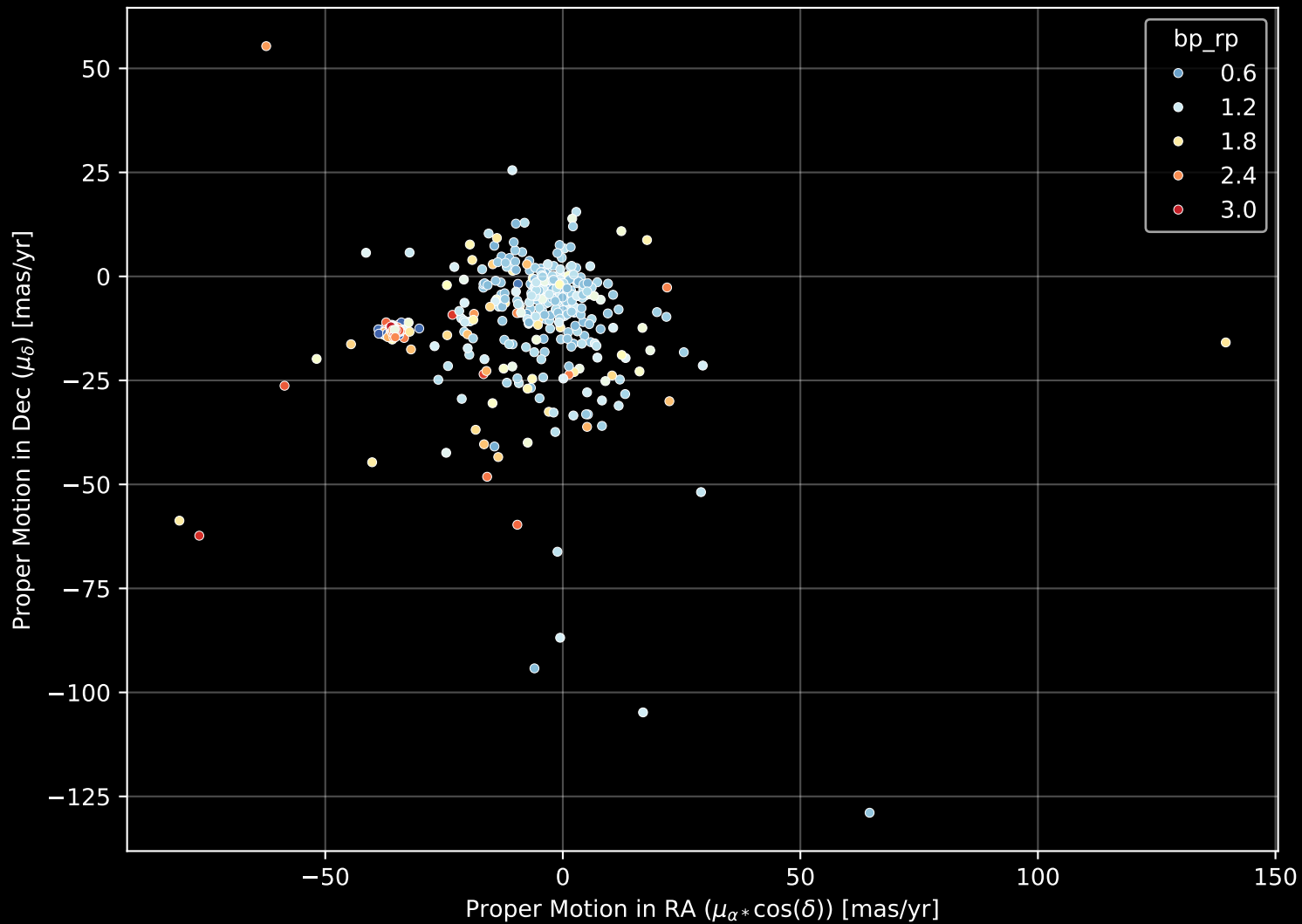
APOGEE DR17 Field: [NGC2632_btx] Proper Motion Diagram (n= 548)
