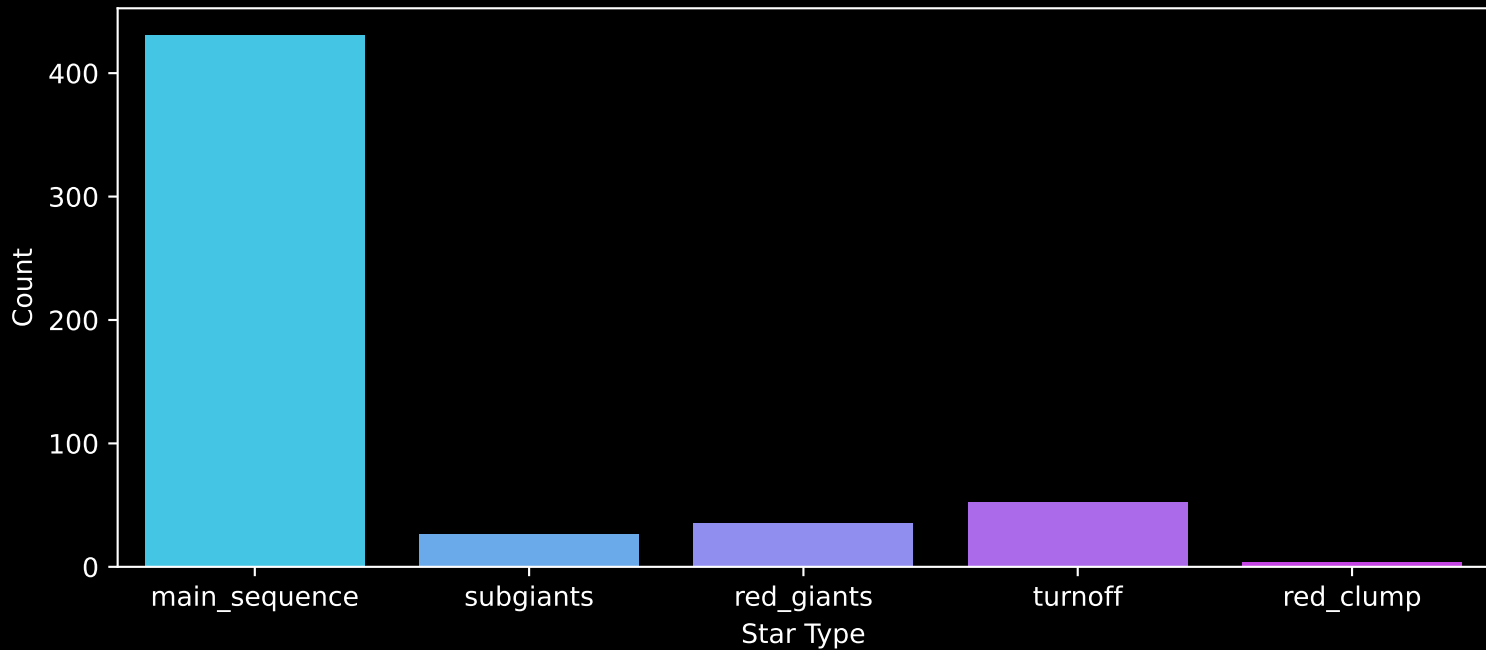
APOGEE DR17 Field: [NGC2632_btx] Count plot of Star Type
