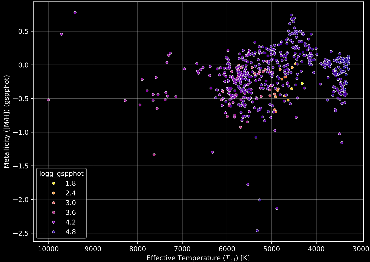
APOGEE DR17 Field: [NGC2632_btx] Stellar Population Parameters (n= 548)
