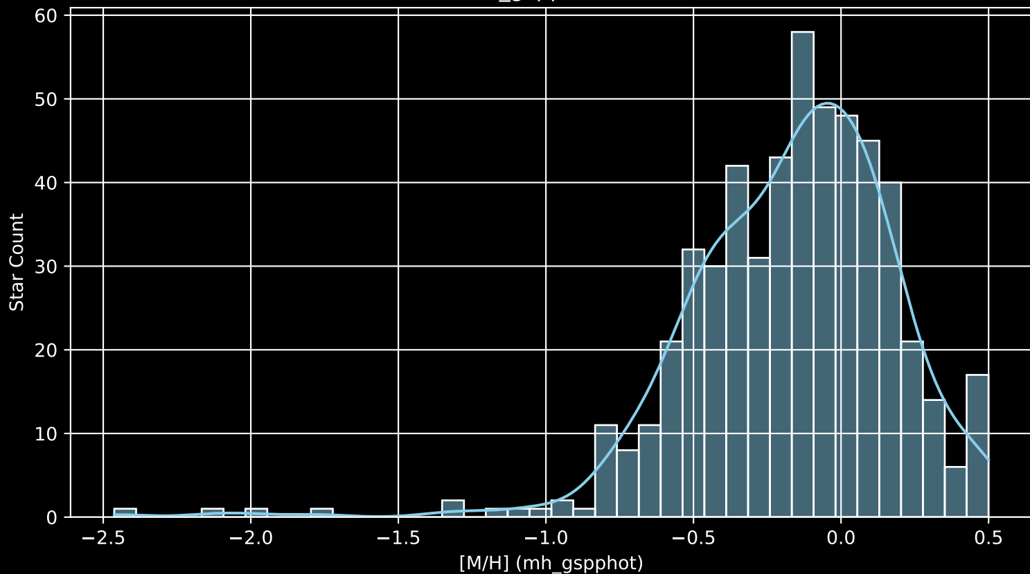
APOGEE DR17 Field: [NGC2632_btx [M/H] (mh_gspphot) (n= 539)
